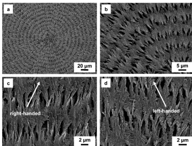
Figure 2. Typical FESEM images of the K_2Cr_2O_7 helical architectures grown in PAA gel matrix without the additives after evaporation of water. (a) Spherulitic morphology. (b) Branches having a helical architecture in the spherulite. (c and d) Right- and left-handed helical forms, respectively.
