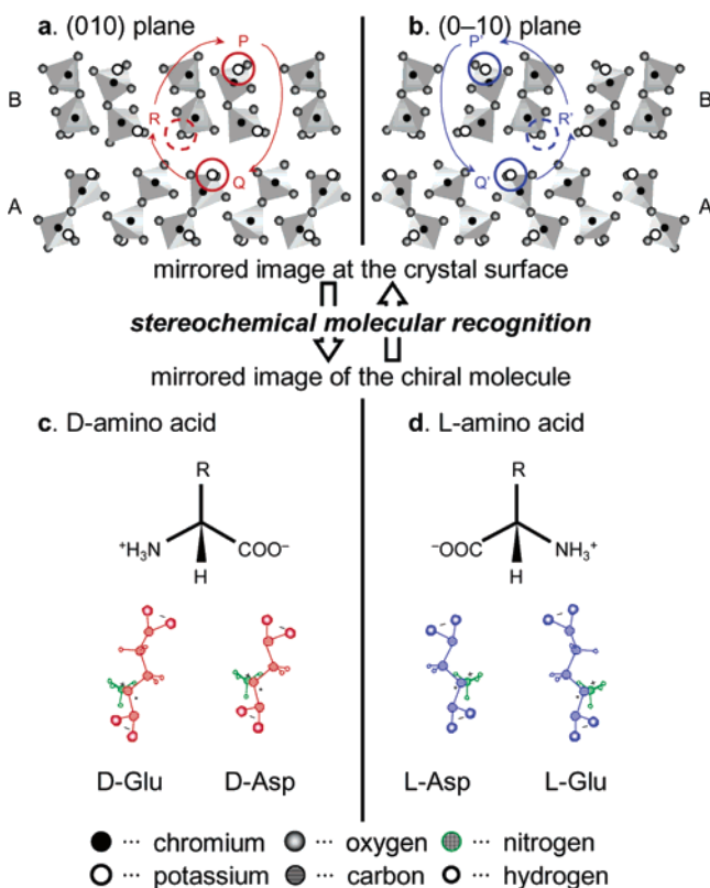
Figure 6. Schematic model for stereochemical recognition between the {010} planes of K_2Cr_2O_7 and chiral molecules. (a and b) The surface cleavage of the (010) and (0-10) planes. (c and d) The structures of the enantiomers for the amino acids.
